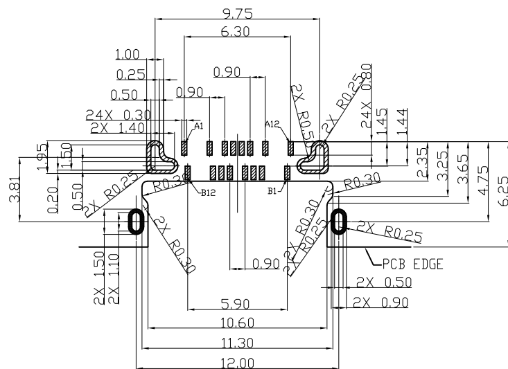
RECOMMENDED PCB LAYOUT (Tolerance=±0.05)
